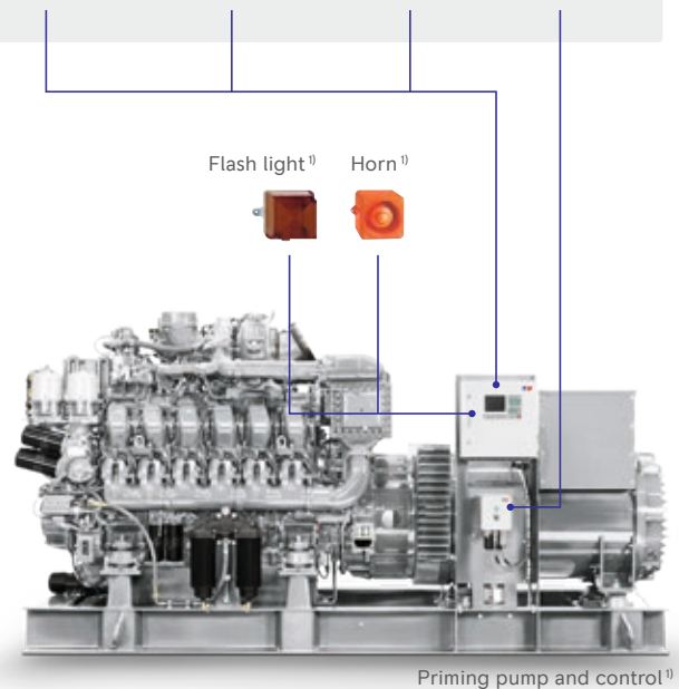
Priming pump and control 1)
